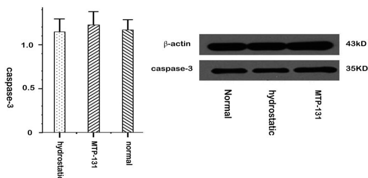
Figure 6. There is no significant difference in the expression of the caspase-3 protein among the three groups (normal group, hydrostatic group, and MTP-131 group) ( p>0.05 ).
